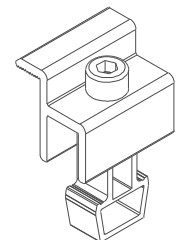
Universal end clamp Material: Aluminum extrusion, 6005 T5 Finish: Clear or black anodized Frame size: 30/40mm
